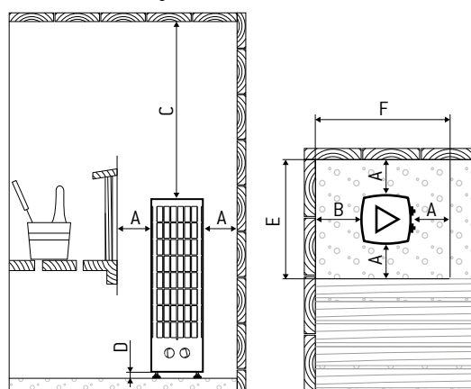
Classic Quatro, safety distances (mm)
