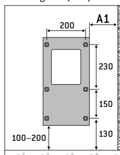
Mounting rack (mm)
